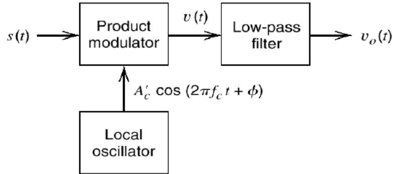
Fig.5 : Coherent detector
