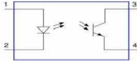
Optocoupler schematic showing LED and phototransistor
