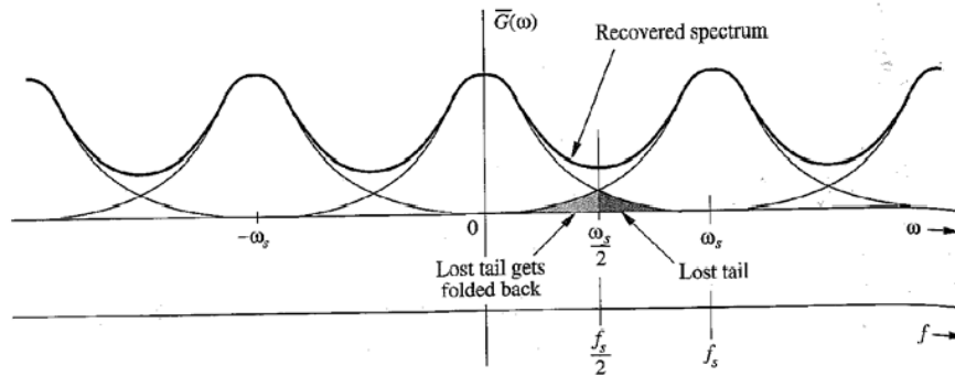
Fig. 1.8 Aliasing effect
