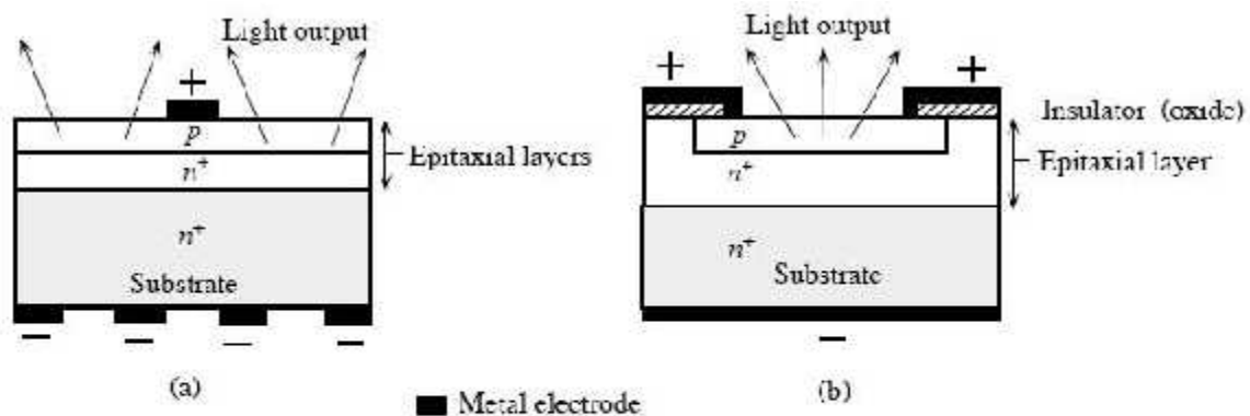
A schematic illustration of typical planar surface emitting LED devices. (a) p-layer grown epitaxially on an n^+ substrate. (b) First n^+ is epitaxially grown and then p region is formed by dopant diffusion into the epitaxial layer.
