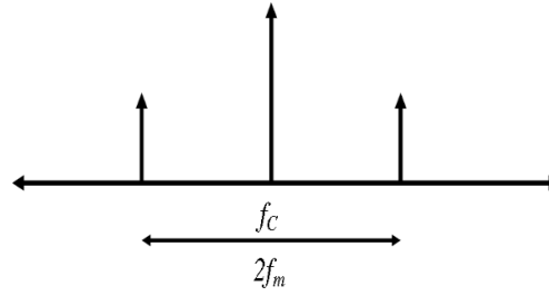
Fig.3. Frequency Domain characteristics of single tone AM
