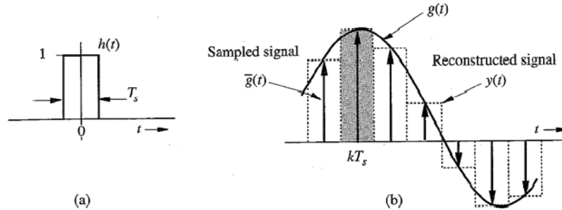
Fig. 1.5 Simple interpolation using zero-order hold circuit
