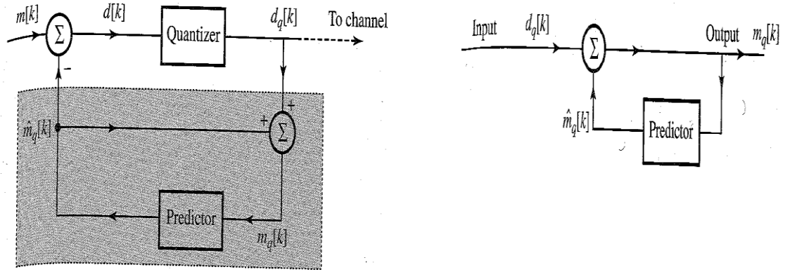
Fig. 2.9 DPCM system – Transmitter and Receiver
