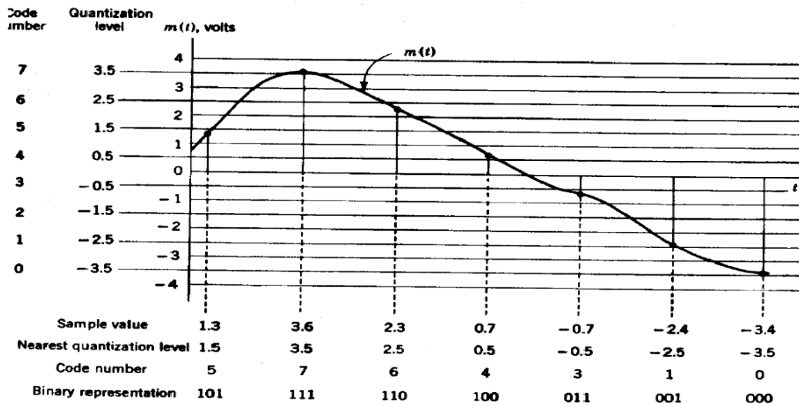
Fig. 2.5 Representation of each sample by its quantized value and binary representation.
