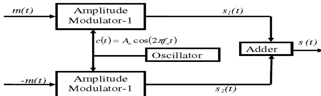
Fig 3 : Balanced modulator
