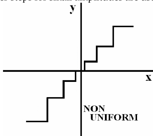
Fig. 2.3. Non-uniform quantization
